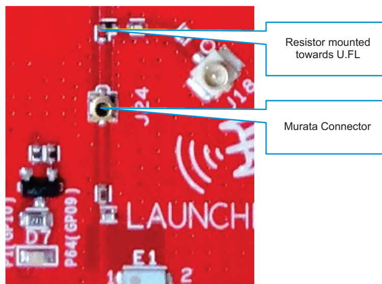
Figure 14. Board Set for Conducted Testing
